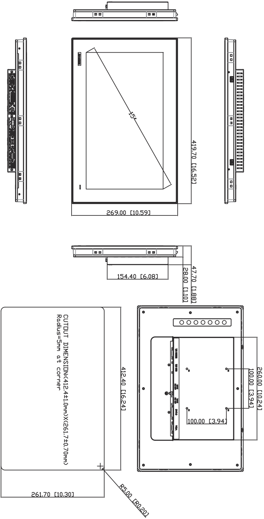
Figure 1.1 FPM-7151W Dimensions
