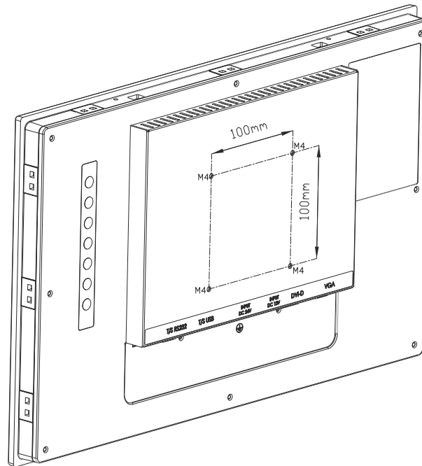
Figure 2.3 VESA Mount
