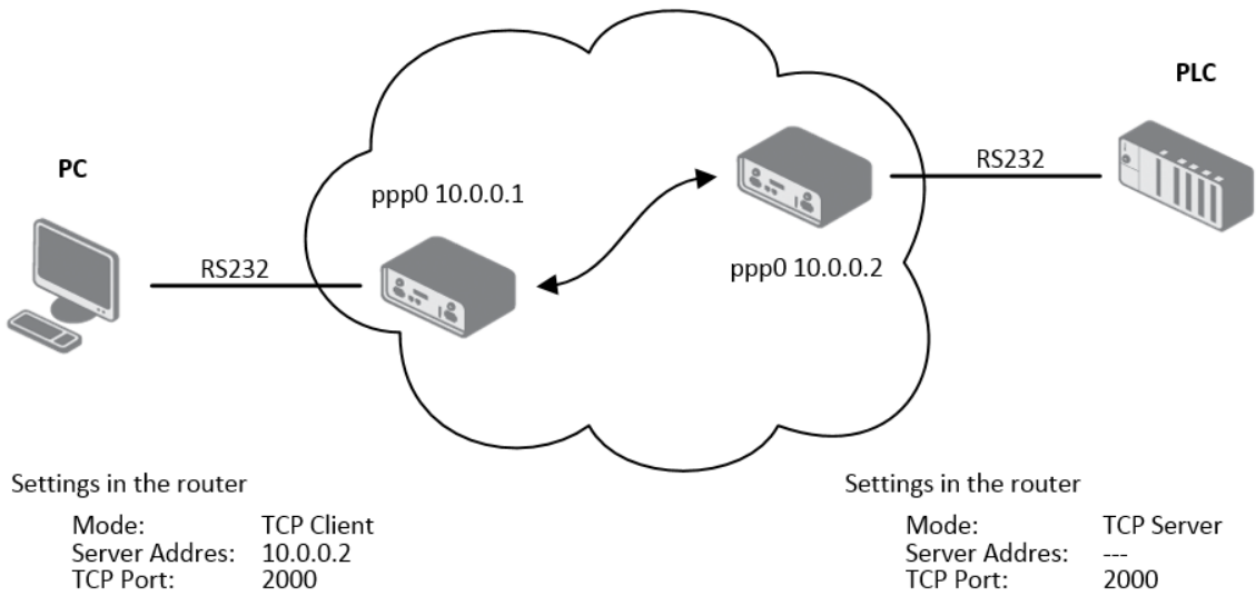
Figure 62: Example of serial port extension
