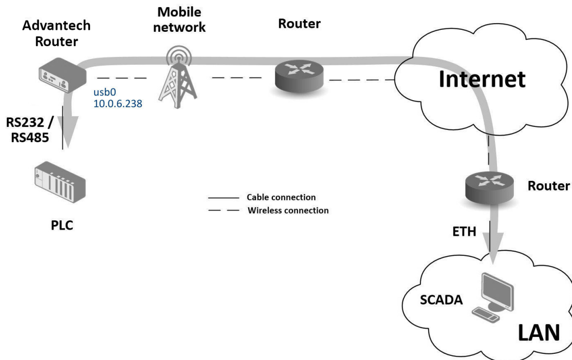
Figure 99: Serial Gateway – sample topology
