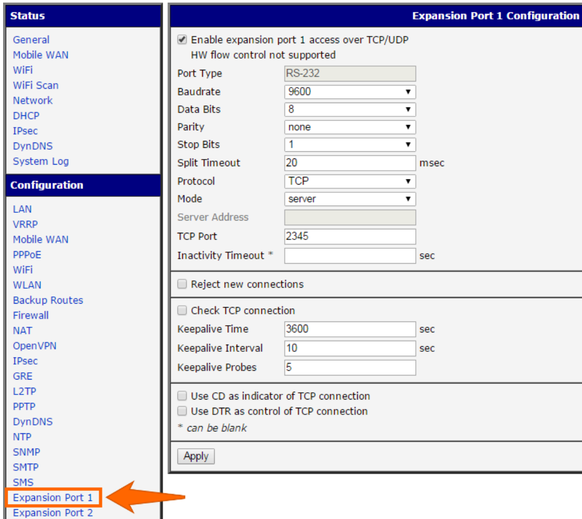
Figure 100: Serial Gateway – konfigurace Expansion Port 1
