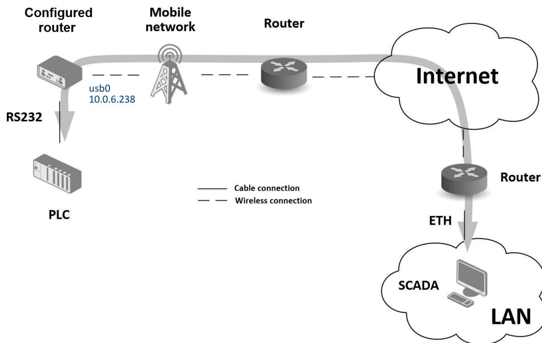
Figure 95: Serial Gateway – sample topology
