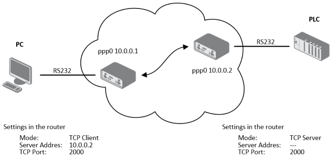
Figure 67: Example of serial interface extension
