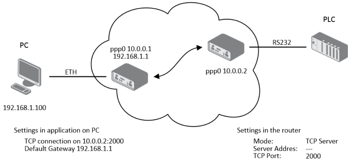
Figure 66: Example of Ethernet to serial communication
