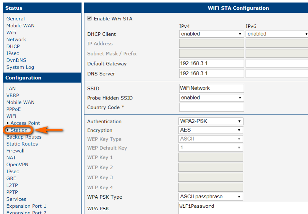
Figure 90: Backup access to the Internet – WiFi configuration
